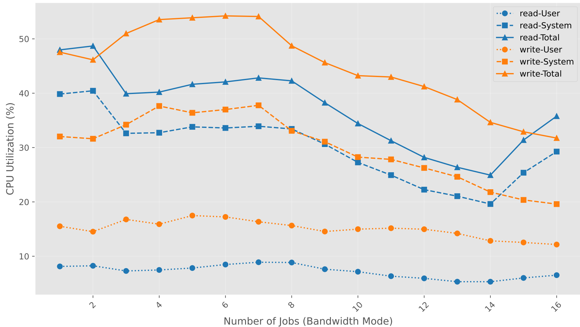
CPU Total vs Number of Jobs (Bandwidth Mode)
